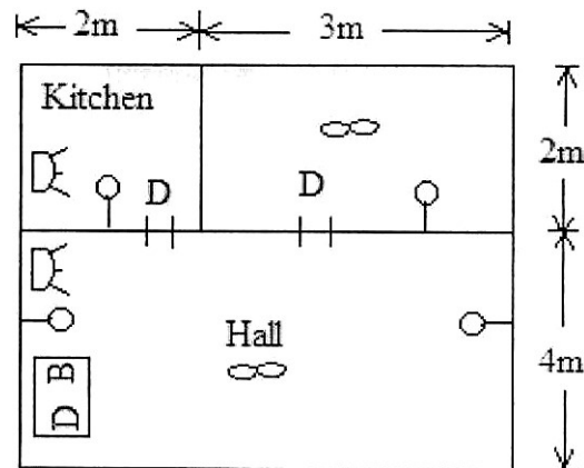
Fig. Plan of house
